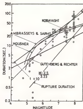
Fig.-5 Duration and Magnitude Proposed by Various Researchers
